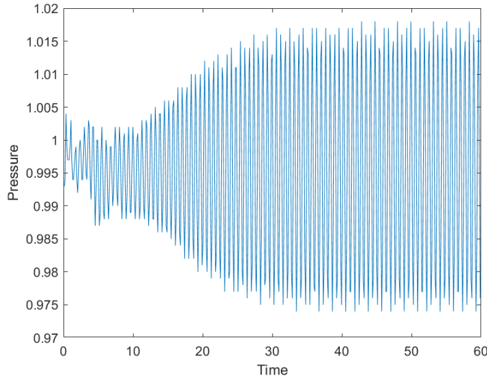
Figure 2: Pressure readings from idealized simulation scenario
