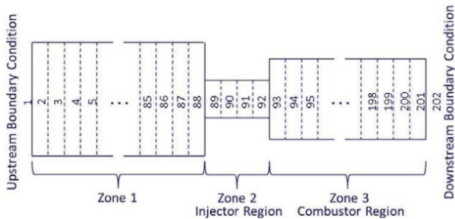
Figure 1: 3-sectored combustor configuration with 202 cells, from “NASA One-Dimensional Combustor Simulation-User Manual for S1D_ML,” 2014 [1]
