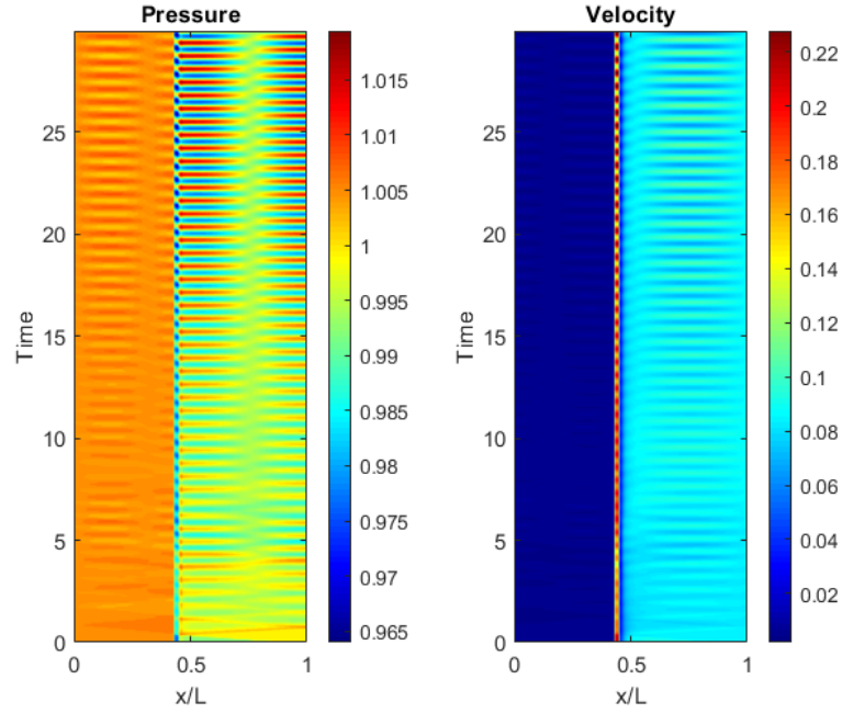
Figure 3: 1-dimensional pressure and velocity data along time
